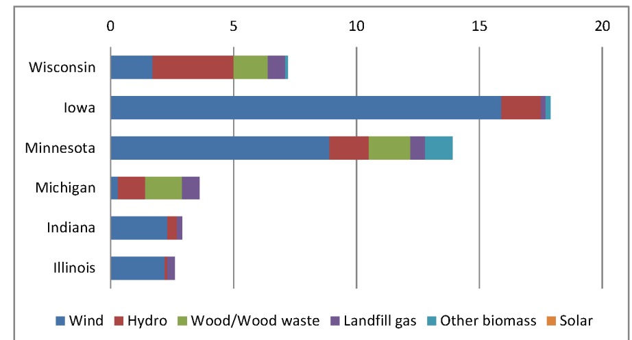
Figure 12: Percentage of Electricity from Renewable Energy in 2010
