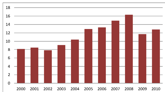
Figure 11: $ Leaving Wisconsin for Energy (Billions)
