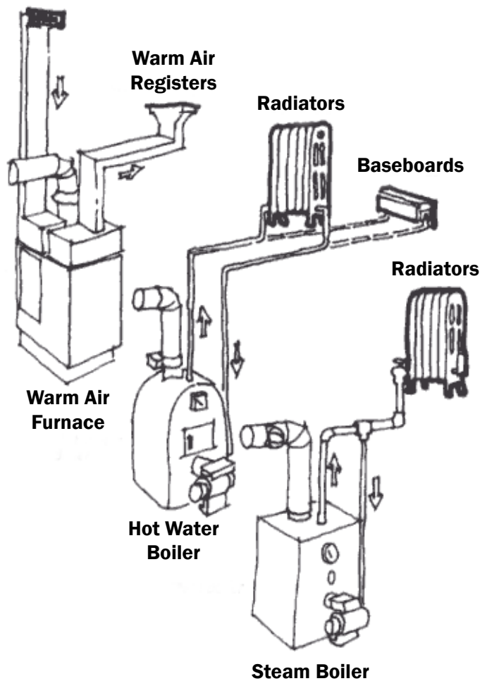
Furnaces heat air, while boilers heat water
