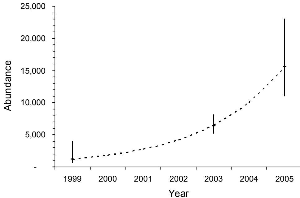
Figure 9. Abundance of lake trout ( \geq 52 cm) in Lake Pend Oreille, Idaho estimated by mark-recapture in 1999, 2003, and 2005 (error bars) and by an exponential growth model fit to the three annual mark-recapture estimates (dashed line; r^2 = 0.99974 ).
