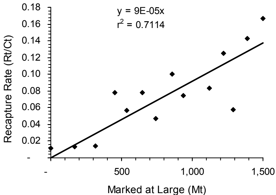
Figure 6. Schumacher-Eschmeyer multiple-census mark-recapture model of the recapture rate of previously marked lake trout ( R_t/C_t ) versus the number of marked lake trout at large ( M_t ) over 14 weekly sampling periods in Lake Pend Oreille, Idaho from September 10, 2005 through December 15, 2005.
