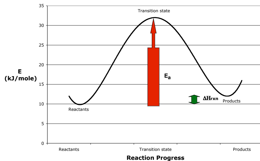
Reaction Potential Energy Diagram: Reversible, Endothermic
