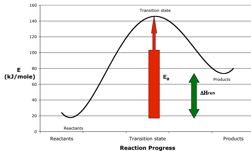
Reaction Potential Energy Diagram: Irreversible, Endothermic
