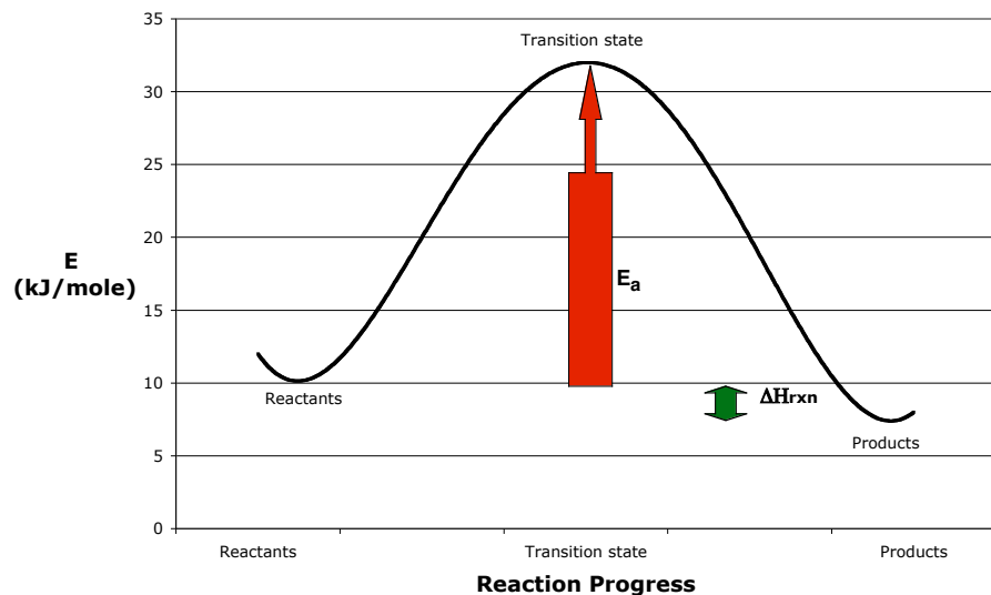
Reaction Potential Energy Diagram: Reversible, Exothermic
