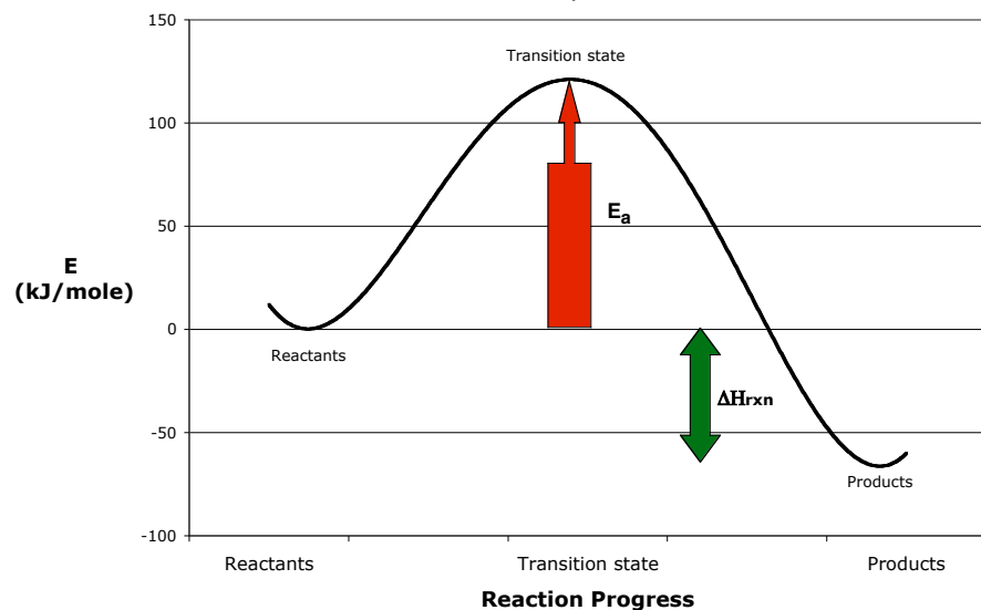
Reaction Potential Energy Diagram: Irreversible, Exothermic
