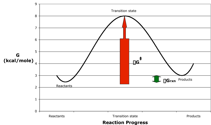
Free Energy Reaction Coordinate Diagram: Reversible, Endergonic
