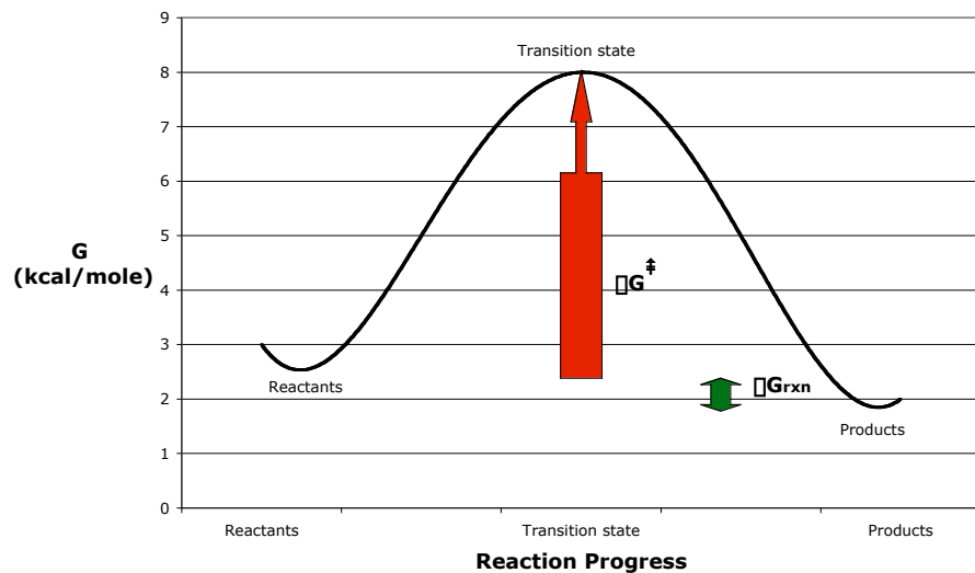
Free Energy Reaction Coordinate Diagram: Reversible, Exergonic
