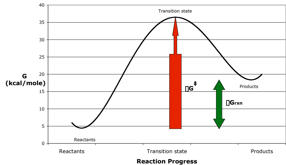
Free Energy Reaction Coordinate Diagram: Irreversible, Endergonic
