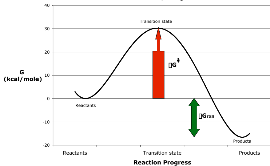
Free Energy Reaction Coordinate Diagram: Irreversible, Exergonic
