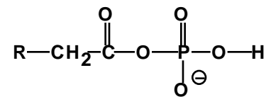
acyl phosphate
