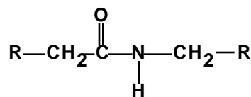
amide linkage
