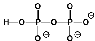
phosphoanhydride
