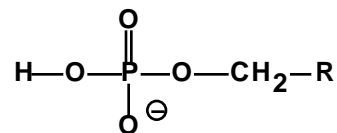
phosphoester
